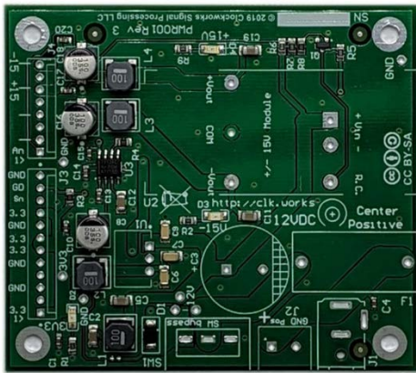
Figure 2 PWR001 with SMT only parts
