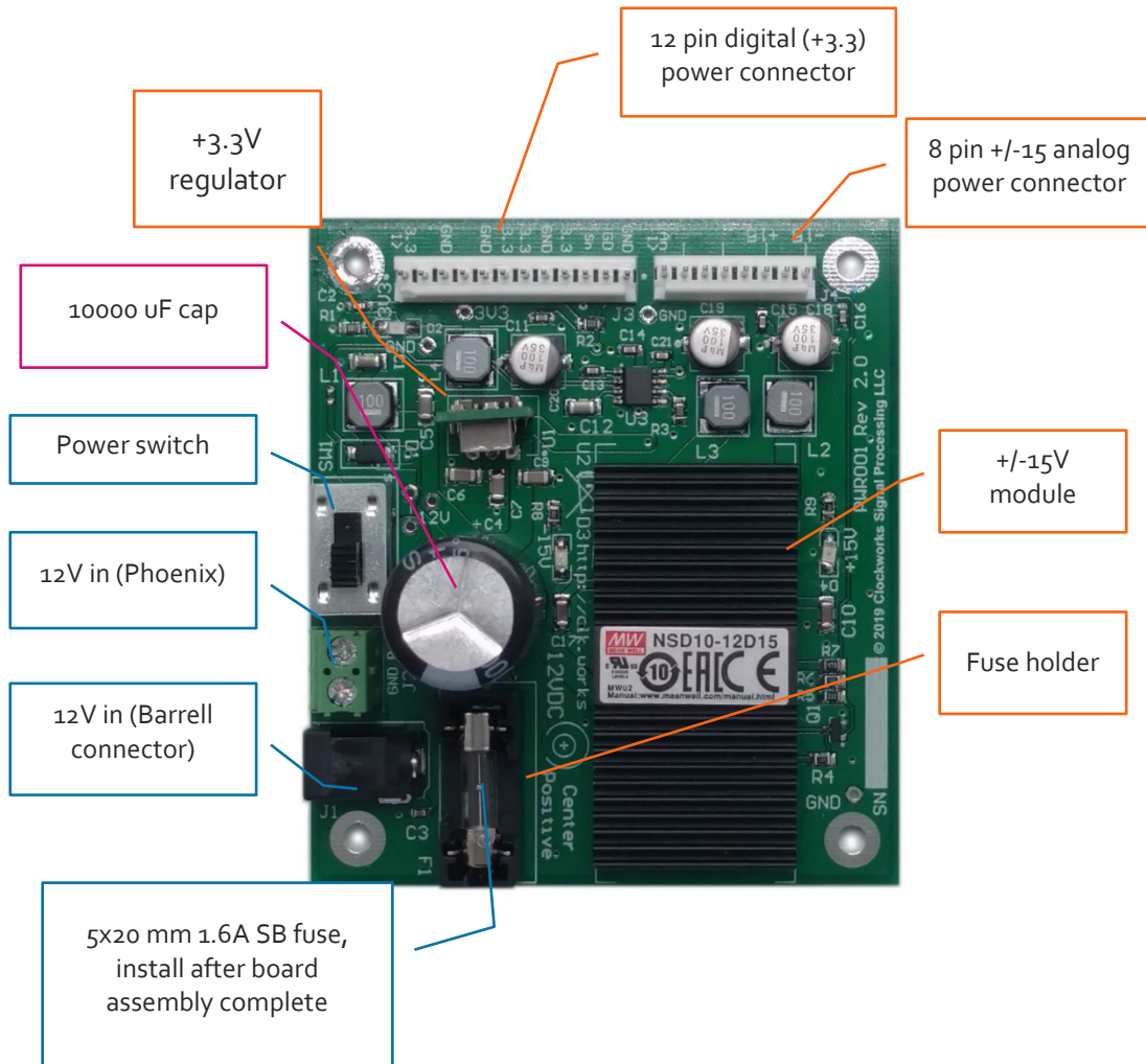
Figure 4 Board part locations for through-hole assembly
